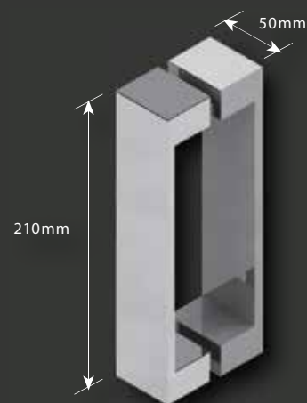
CUBIX50 - Double Pull Handle
