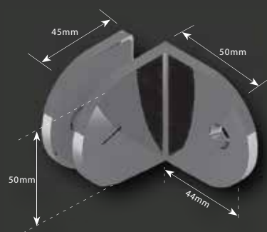
SB50 - Wall Fix Shower Bracket
