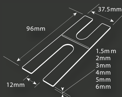
PP1.5/PP2/PP3/PP4/PP5/PP6 - Plastic Packers
