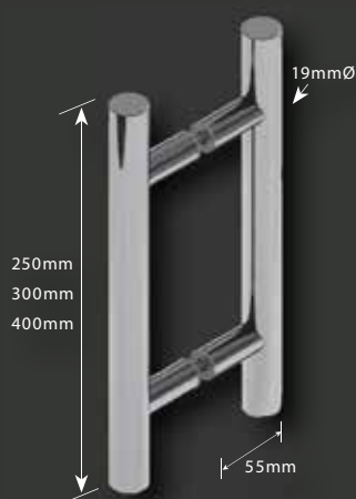
HM150/210/300 - Marsh Handle
