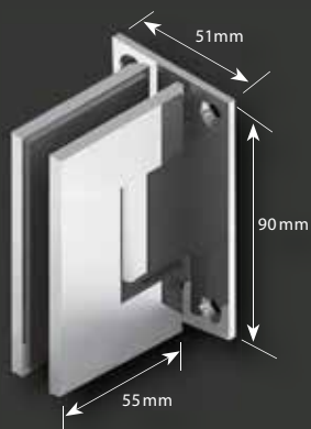
ES1 - Wall Hung Hinge
