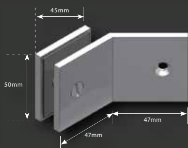
SB135SQ - Square Wall Fix Shower Bracket
