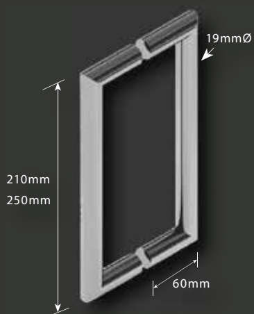
MATISSE H01/H02 - Double Pull Handle
