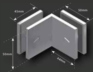
SBD50SQ - Glass to Glass Fix Shower Bracket - Double sided
