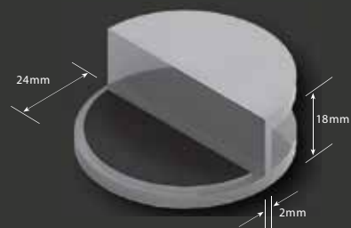
SB10STOP - Shower Door Stop
