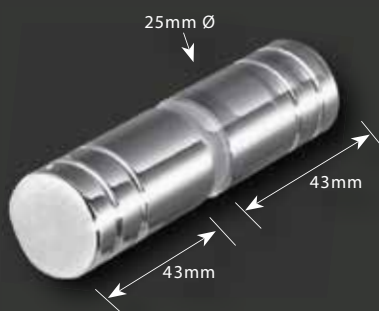
SK40 - Double Pull Knob
