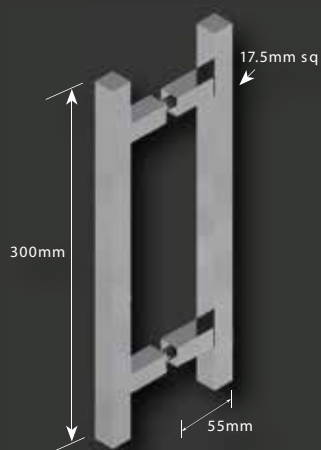
HM210SQ - Marsh Square Handle
