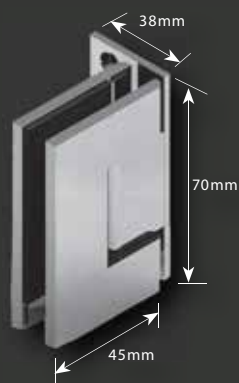
CMES1L - Wall Hung Hinge Single Side
