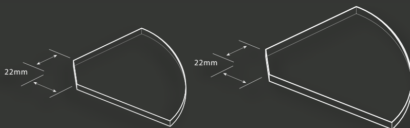
GS200CFL/GS200LOW and GS250CFL/GS250LOW - Corner Glass Shelf
