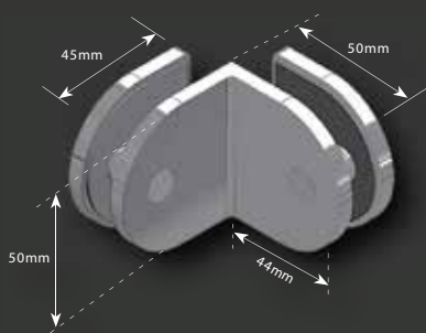
SBD50 - Glass to Glass Fix Shower Bracket - Double sided
