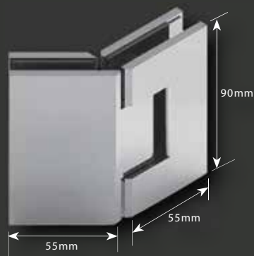
ES2-135 - Glass to Glass 135° Hinge
