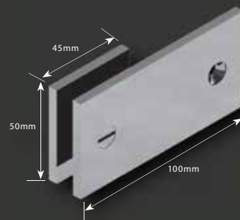
SB180SQ - Square Wall Fix Shower Bracket
