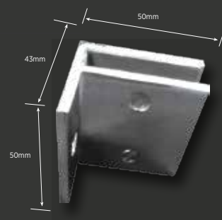
SB50NHSQ - Square Glass Shelf Bracket
