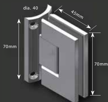
CMES1-RP - Glass to Round Post
