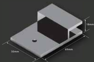
SB10VLSQ - Square Glass Shelf Bracket
