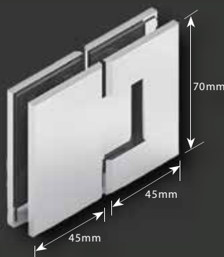
CMES2 - Glass to Glass
