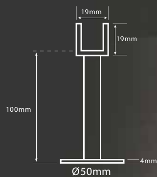
SSB100 - Shower Bracket Support
