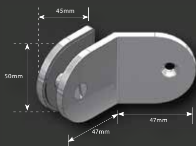
SB135 - Wall Fix Shower Bracket
