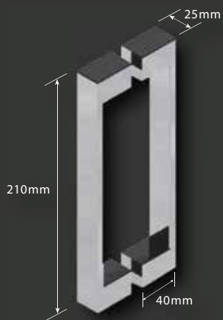
CUBIX25 - Double Pull Handle
