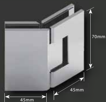
CMES2-135 - Glass to Glass 135° Hinge
