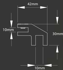
OPF2 - Overpanel Fitting
