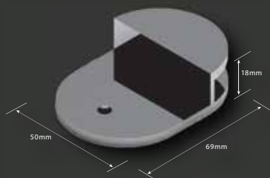
SB10VL - Glass Shelf Bracket
