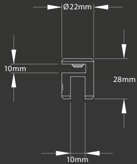
OPFIRD - Overpanel Fitting
