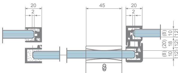
Art. 4-020 Brush seal
