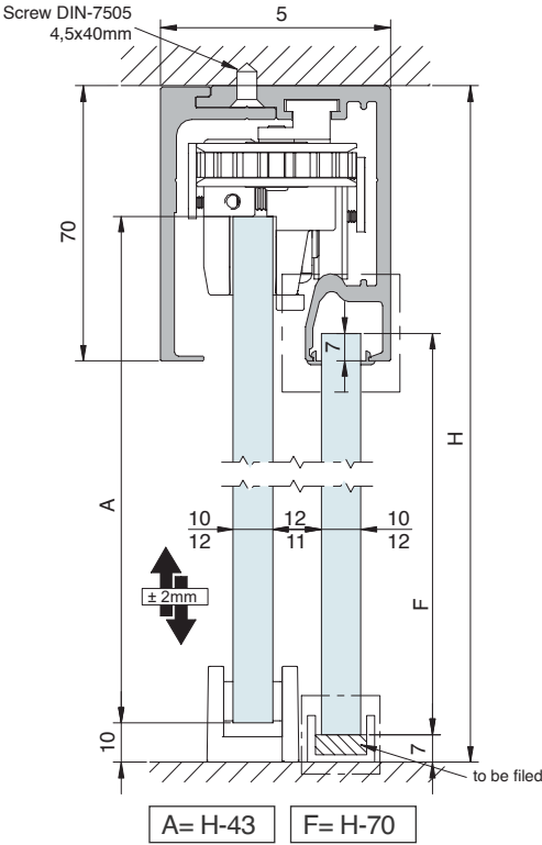
TRACK 3 Wall / Ceiling mount with fixed panel
