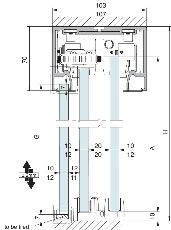
TRACK 1 and 2 Ceiling mount with fixed glass
